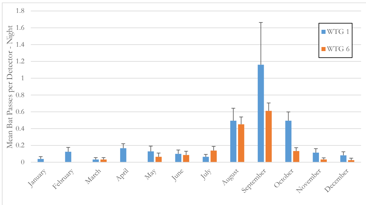
Figure 3-5. Acoustic data by month from ground detectors, 2013-2016.
